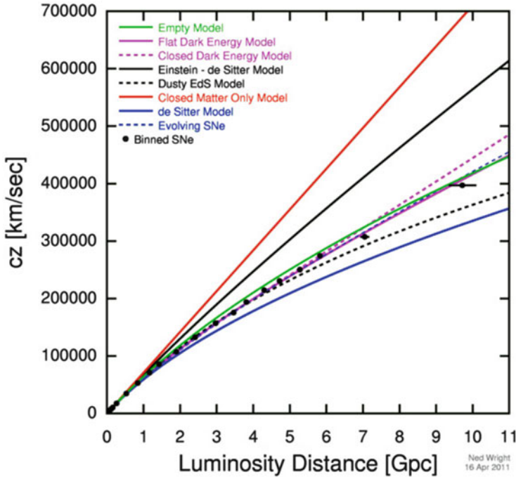
Fig. 4 Here, the differences in the magnitude-redshift relation for different cosmological models are shown. The supernova data can best be fitted by a model with \Omega_{\Lambda} = 0.7, \Omega_{tot.} = 1 , the magenta colored line (Source: Legacy supernova survey ( http://www.cfht.hawaii.edu/SNLS/ ) [4])
